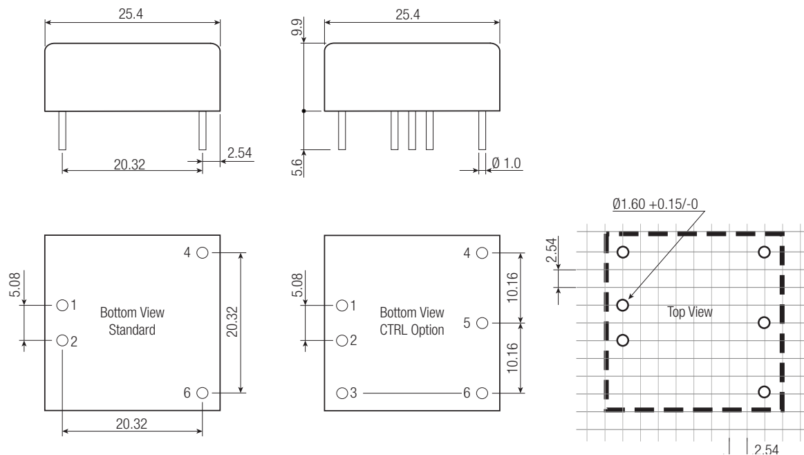
Dimension Drawing (mm)
