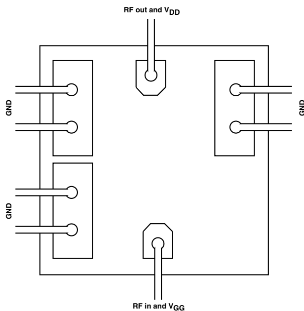
BONDING LAYOUT
