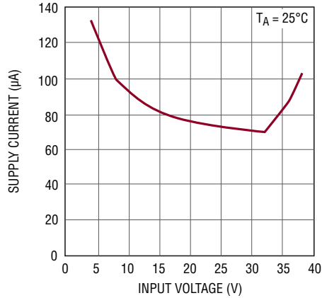
No-Load Supply Current vs V_{IN}
