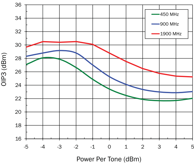
OIP3 versus Power Out ( V_d = 3V , 25C)
