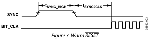
Figure 3. Warm \overline{RESET}
