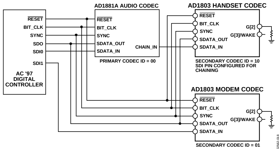
Figure 18. Codec Chaining Allows Several Analog Devices AC '97 Codecs to be Connected to One AC Link Controller Port
