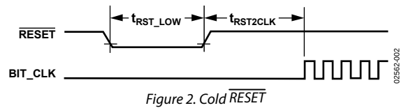
Figure 2. Cold \overline{RESET}
