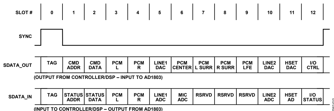
Figure 10. AC '97 Interface Timing
