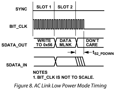
Figure 8. AC Link Low Power Mode Timing
