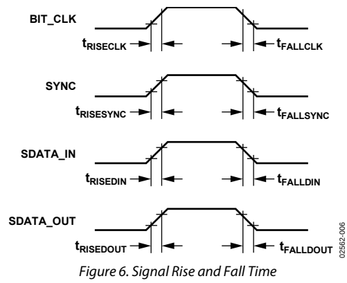
Figure 6. Signal Rise and Fall Time
