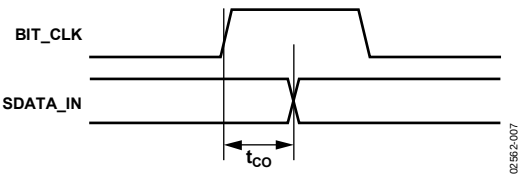
Figure 7. Propagation Delay
