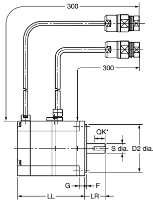
R7M-AP□□□30-BS1-D (With brake)
