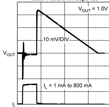
50 \mu\text{s/DIV} Figure 16.
