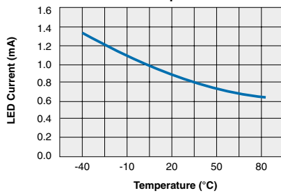
CPC1962 Typical I_F for Switch Operation vs. Temperature
