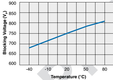
CPC1962 Typical Blocking Voltage vs. Temperature
