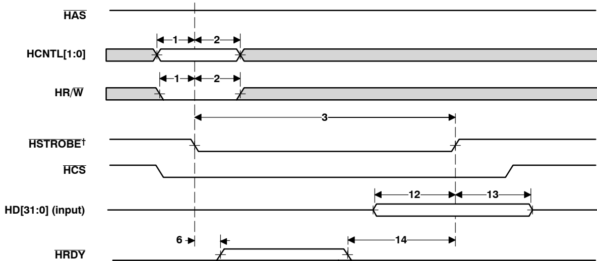
Figure 45. HPI32 Write Timing ( \overline{HAS} Not Used, Tied High)
