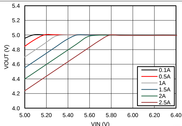
Figure 70. Dropout Curve
