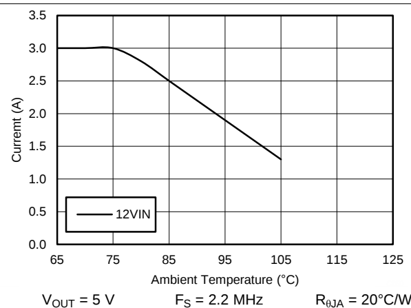
Figure 90. Derating Curve
