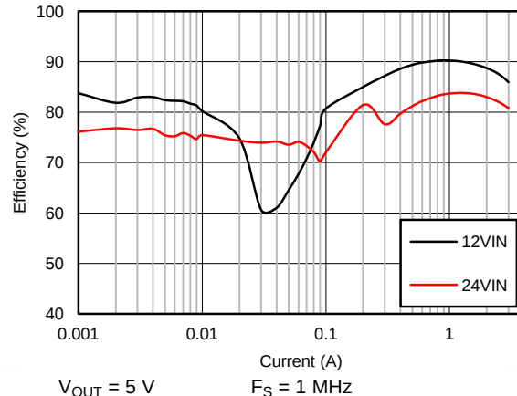
Figure 80. Efficiency
