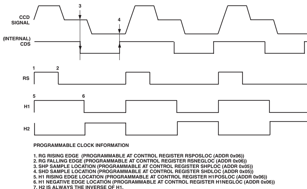
Figure 13. High Speed Clock Programmable Locations
