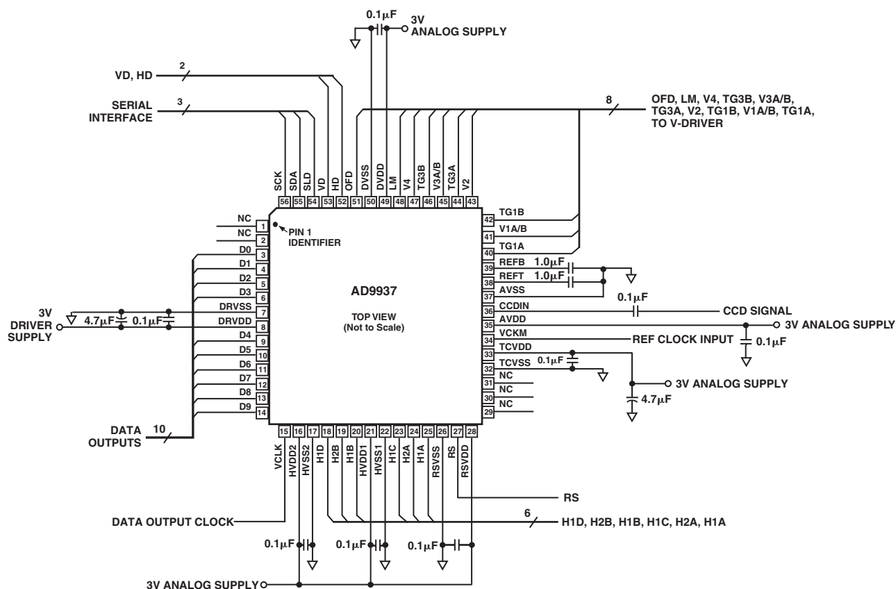
Figure 41. Typical Circuit Configuration
