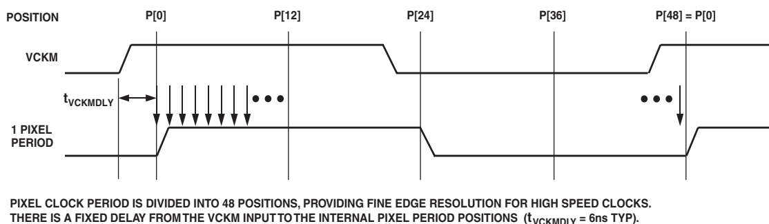
Figure 12. High Speed Clock Resolution from VCKM Master Clock
