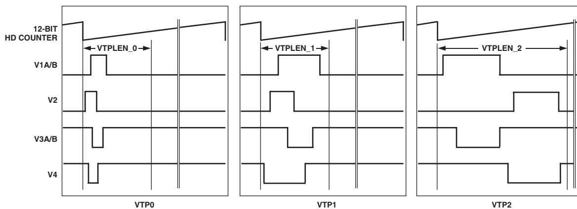
Figure 34. Example of Three Preprogrammed VTP Pulses
