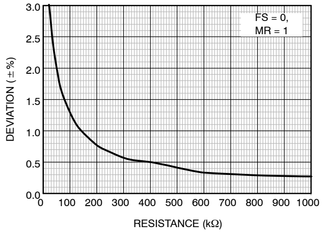
Figure 7. Deviation vs SSEXTR Chart (CLKIN = 15 MHz)
