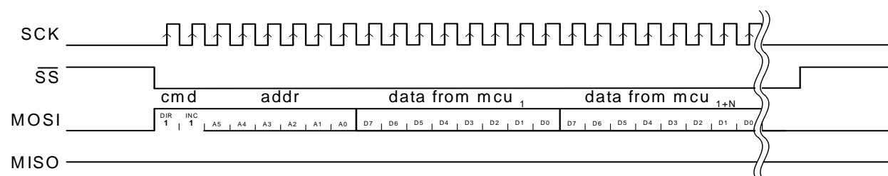
Figure 4. SPI Burst Write Sequence
