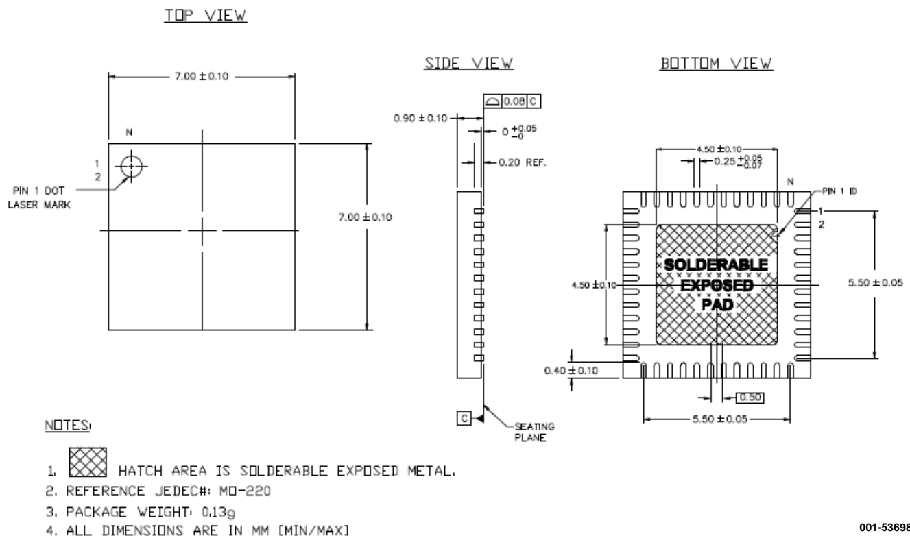
Figure 19. 48-pin QFN 7 x 7 x 1.0 mm LT48C (Sawn)
