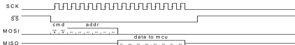
Figure 2. SPI Burst Read Sequence
