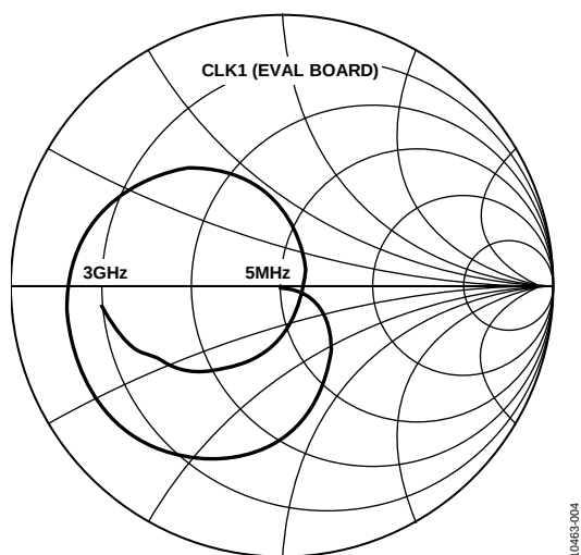
Figure 4. CLK1 Smith Chart (Evaluation Board)
