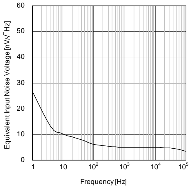
Figure 19. Equivalent Input Noise Voltage vs Frequency ( V_{CC}/V_{EE}=\pm 15V , T_A=25^\circ C , A_V=40dB )
