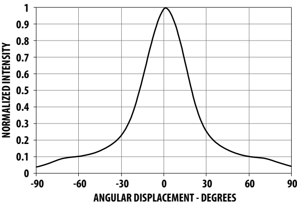
Figure 6 Radiation Pattern for RED – Minor Axis
