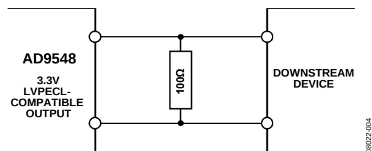
Figure 29. DC-Coupled LVDS or LVPECL Output Driver
