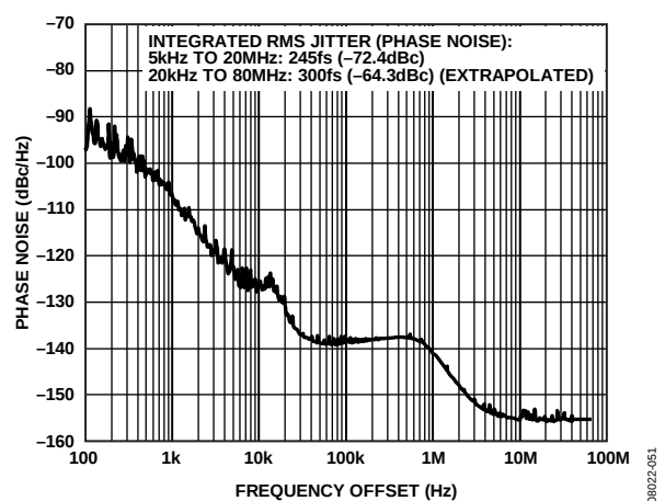
Figure 12. Additive Phase Noise (Output Driver = LVPECL), f_R = 19.44 MHz, f_O = 155.52 MHz, LBW = 1 kHz, f_{SYS} = 50 MHz (Crystal), PLL On with 2x Frequency Multiplier, I_{CP} = 375 \mu A, LF = External (350 kHz)
