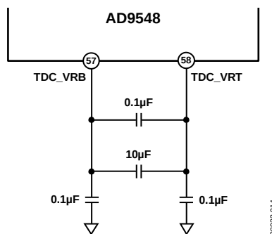
Figure 40. TDC Pin Connections
