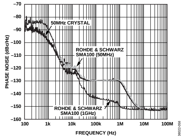
Figure 10. Additive Phase Noise Comparison of SYSCLK Input Options (Output Driver = LVPECL), f_R = 19.44 MHz, f_O = 311.04 MHz, LBW = 1 kHz
