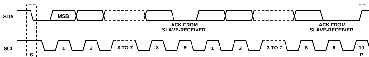
Figure 64. Acknowledge Bit
