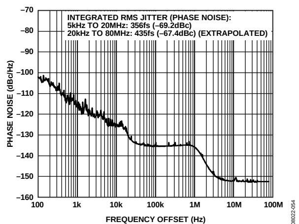
Figure 11. Additive Phase Noise (Output Driver = LVPECL), f_R = 1 Hz, f_O = 155.52 MHz, LBW = 0.05 Hz, f_{SYS} = 50 MHz, PLL On
