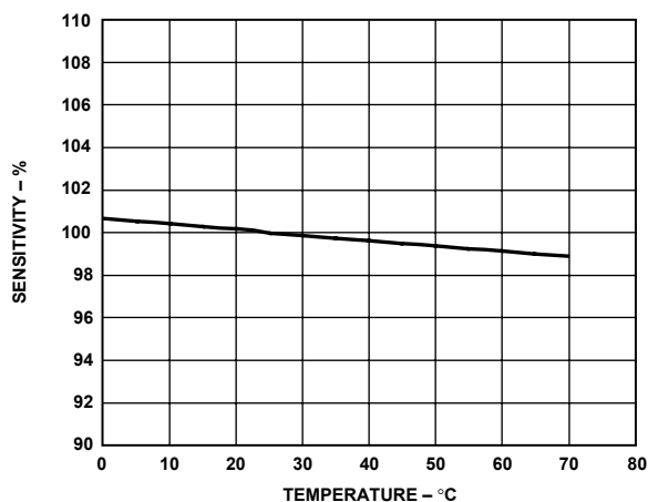
Figure 6. Normalized Sensitivity vs. Temperature
