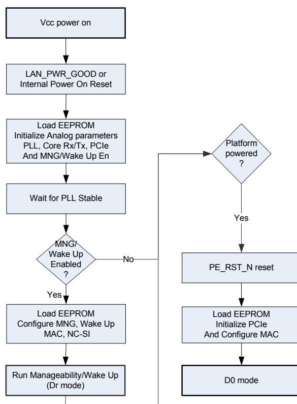
Figure 3-11. 82598 Power-Up Sequence
