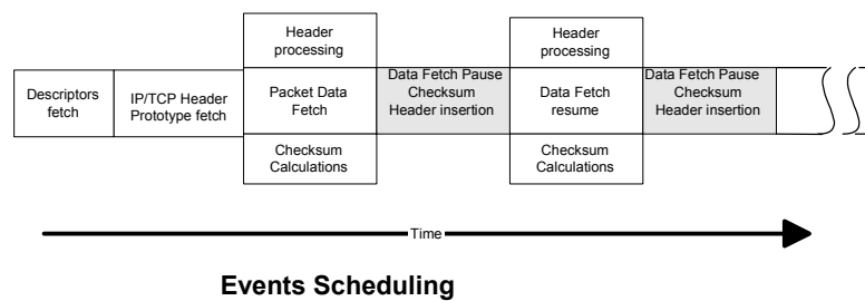
TCP Segmentation Data Flow
