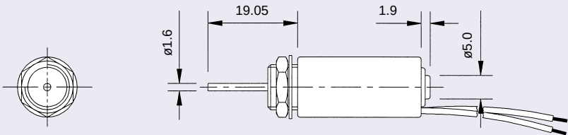
Pull type - shown energised
