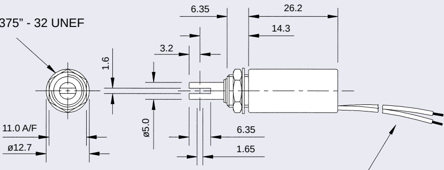
Pull type - shown energised
