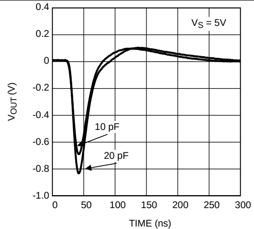
Figure 58. Capacitive Load Response at 5.0 V
