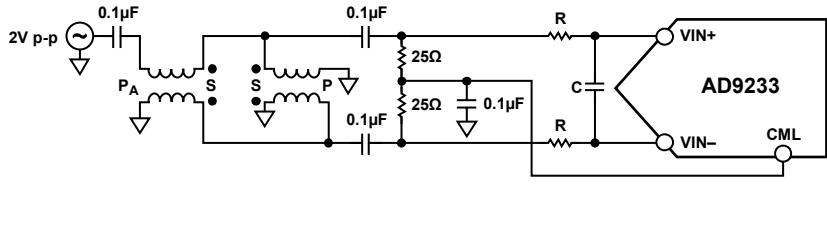
Figure 39. Differential Double Balun Input Configuration
