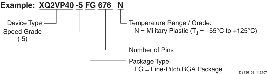
Figure 2: QPro Virtex-II Pro Ordering Example, Wire-Bond Package
