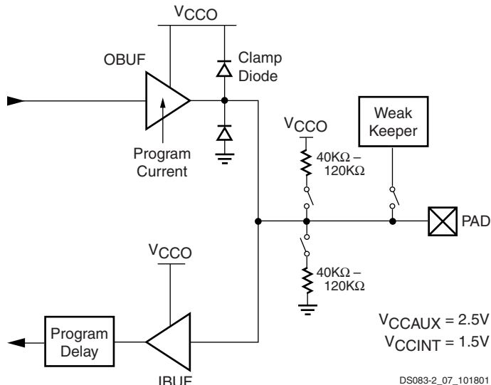
Figure 10: LVTTL, LVCMOS, or PCI SelectIO-Ultra Standard
