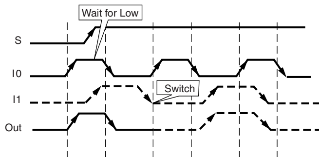
Figure 49: Clock Multiplexer Waveform Diagram
