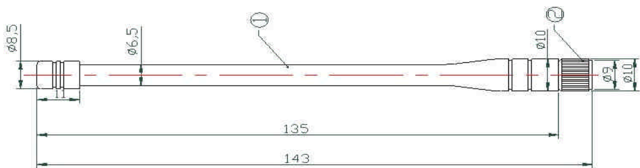
Figure 3 straight SMA
