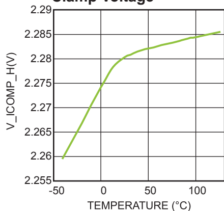
ICOMP High-Level Clamp Voltage
