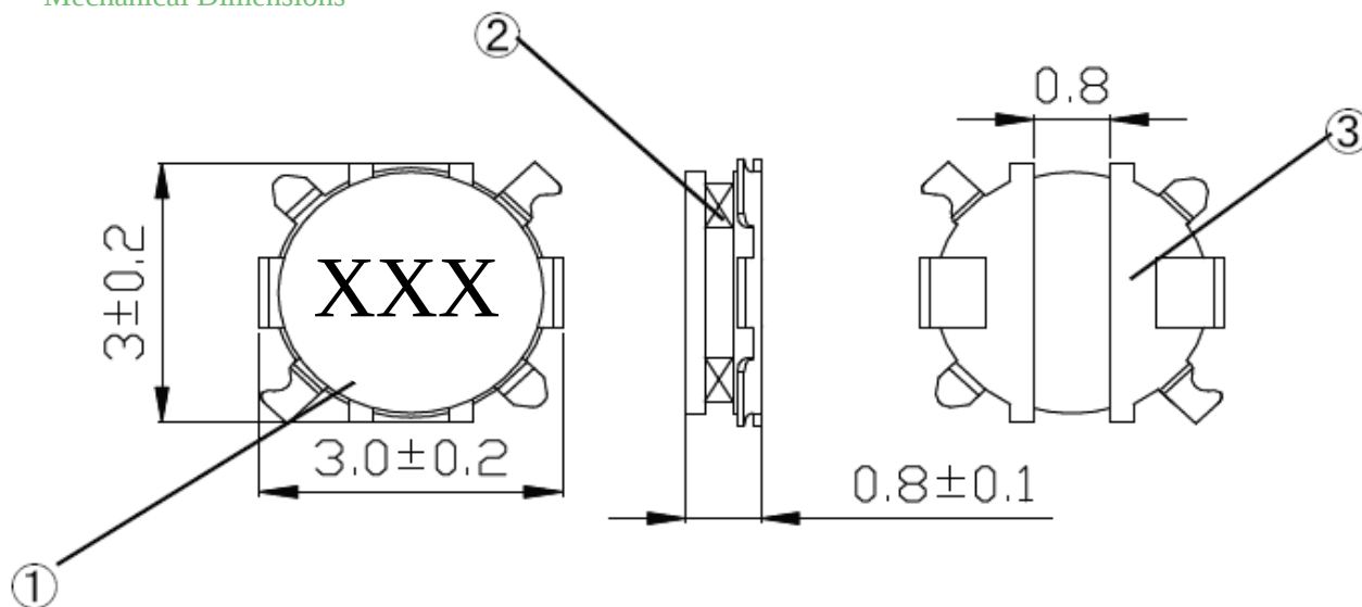
Mechanical Dimensions
