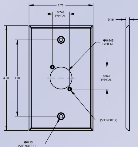
SINGLE GANG 1 CONNECTOR HOLE
