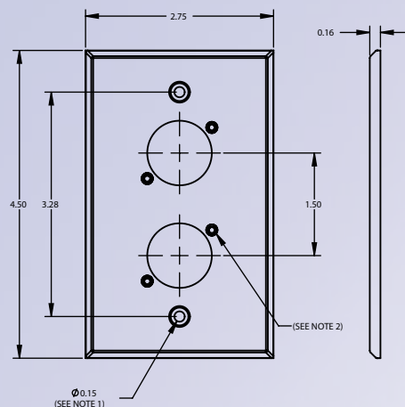
SINGLE GANG 2 CONNECTOR HOLES
