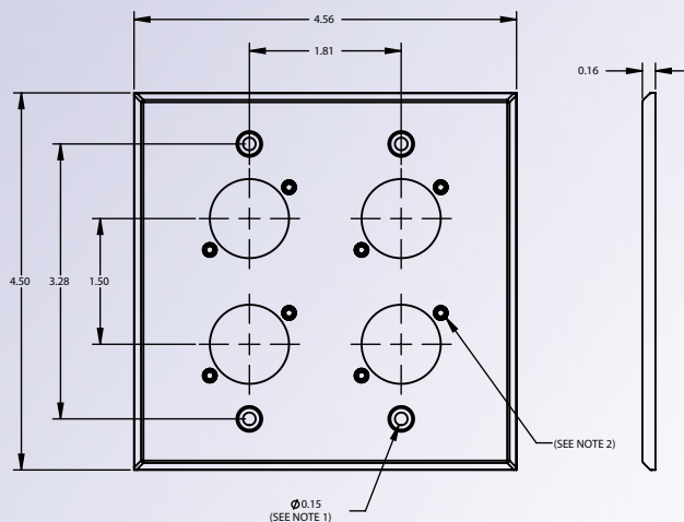
DOUBLE GANG 4 CONNECTOR HOLES
