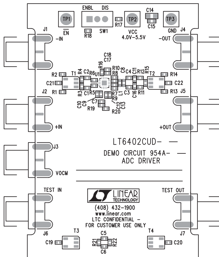
Top Silkscreen
