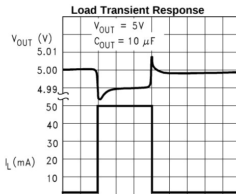
10 \mu\text{s}/\text{div} → Figure 21.
