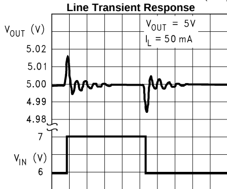
20 \mu\text{s}/\text{div} → Figure 16.
