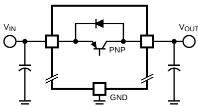
Figure 37. LP2980 Reverse Current Path
