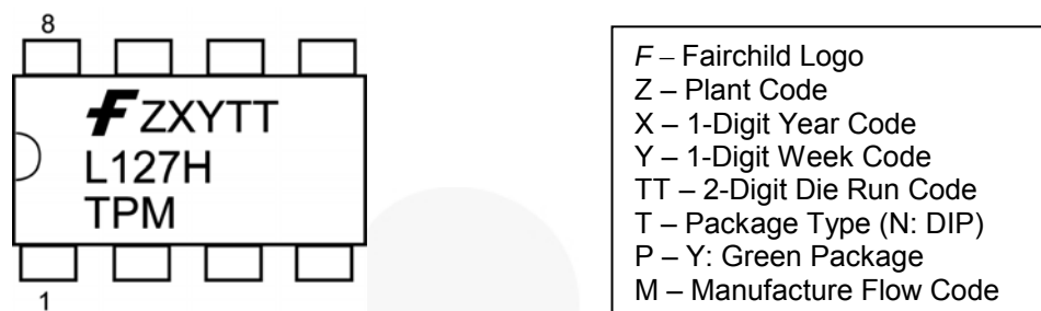
Figure 3. Pin Configuration
