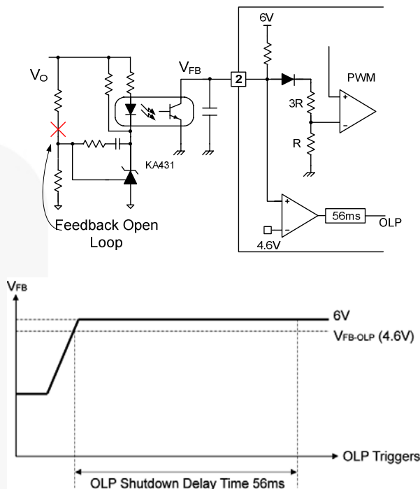
Figure 29. OLP Operation
