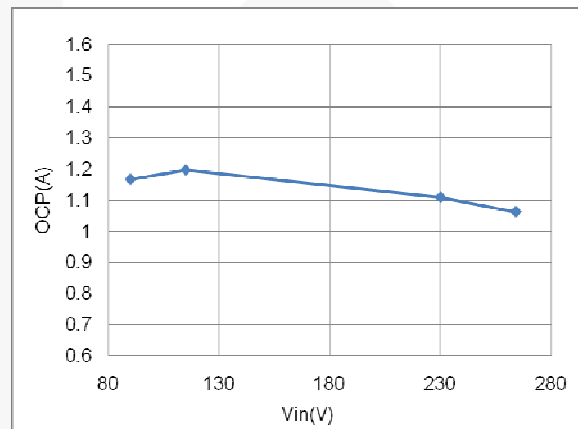
Figure 31. Over-Current Protection
