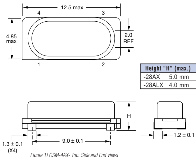
Figure 1) CSM-4AX- Top, Side and End views
