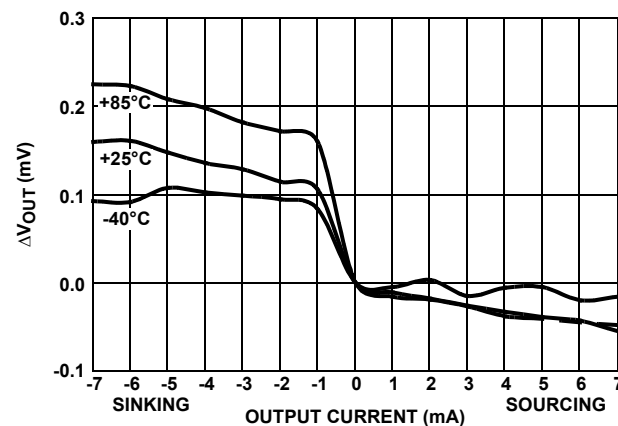
FIGURE 37. LOAD REGULATION
