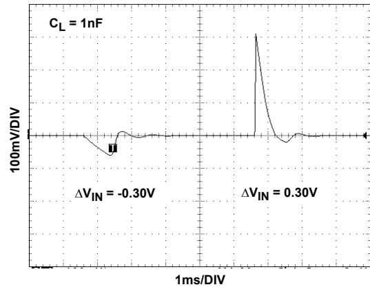
FIGURE 76. LINE TRANSIENT RESPONSE
