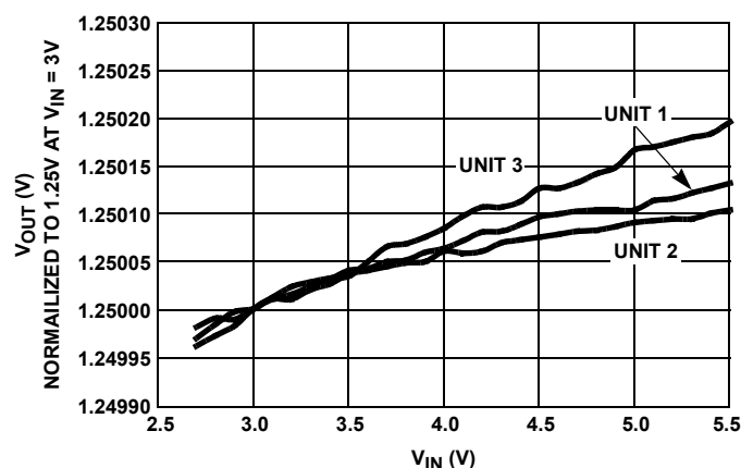
FIGURE 32. LINE REGULATION, 3 UNITS
