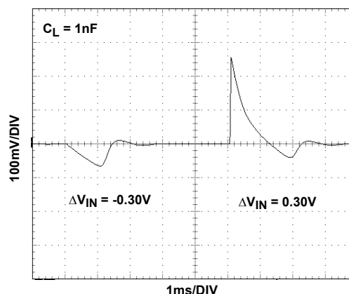
FIGURE 105. LINE TRANSIENT RESPONSE
