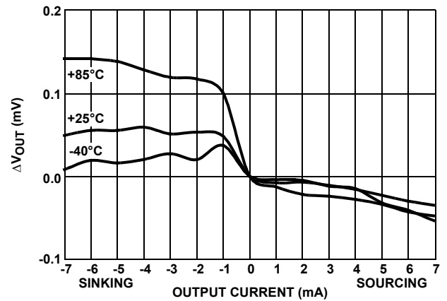
FIGURE 78. LOAD REGULATION OVER-TEMPERATURE
