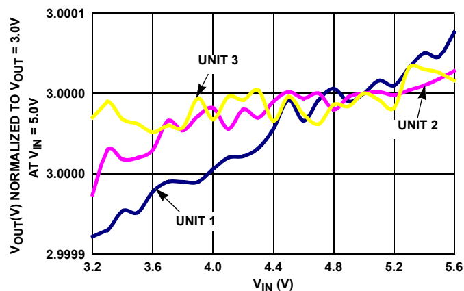
FIGURE 87. LINE REGULATION (3 REPRESENTATIVE UNITS)
