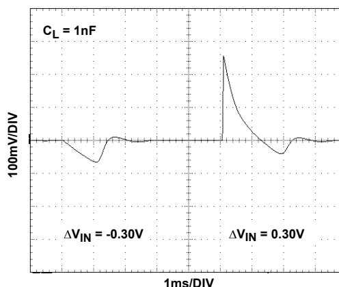
FIGURE 90. LINE TRANSIENT RESPONSE
