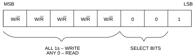
COMMAND WORD Figure 4
