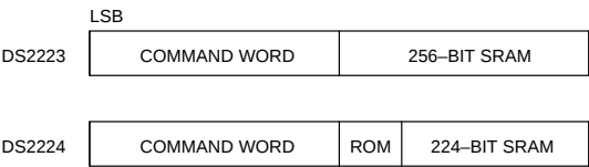
READ/WRITE TRANSACTION Figure 5
