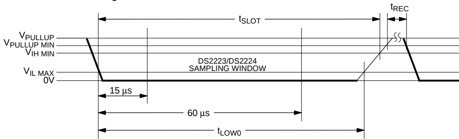
Write-Zero Time Slot Figure 2
