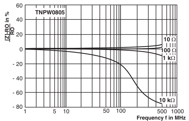
HF Performance
