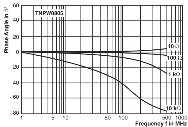
HF Performance
