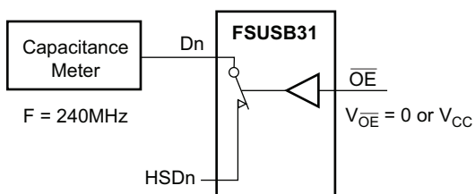
Figure 18. Channel On Capacitance
