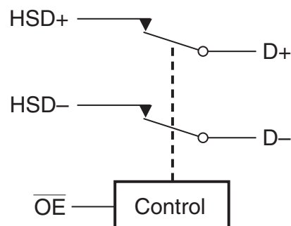
Figure 4. Analog Symbol
