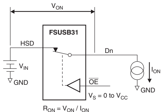
Figure 8. On Resistance
