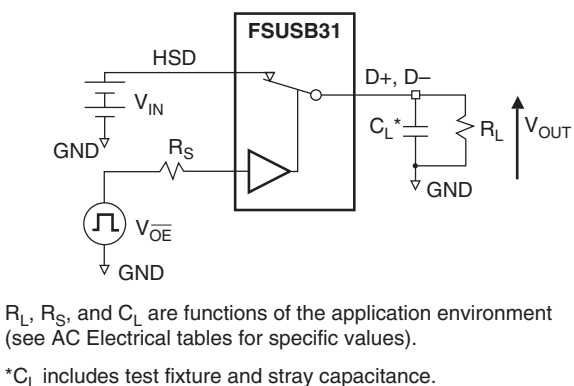
Figure 10. AC Test Circuit Load
