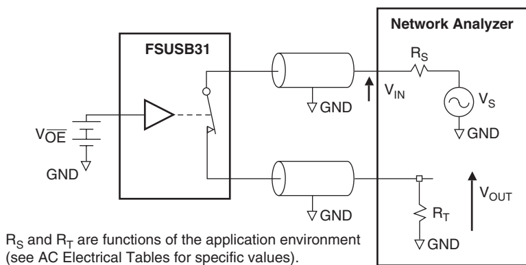
Figure 15. Bandwidth
