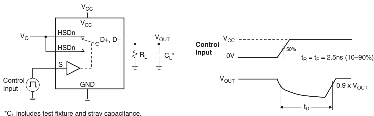
Figure 13. Break-Before-Make ( t_{BBM} )
