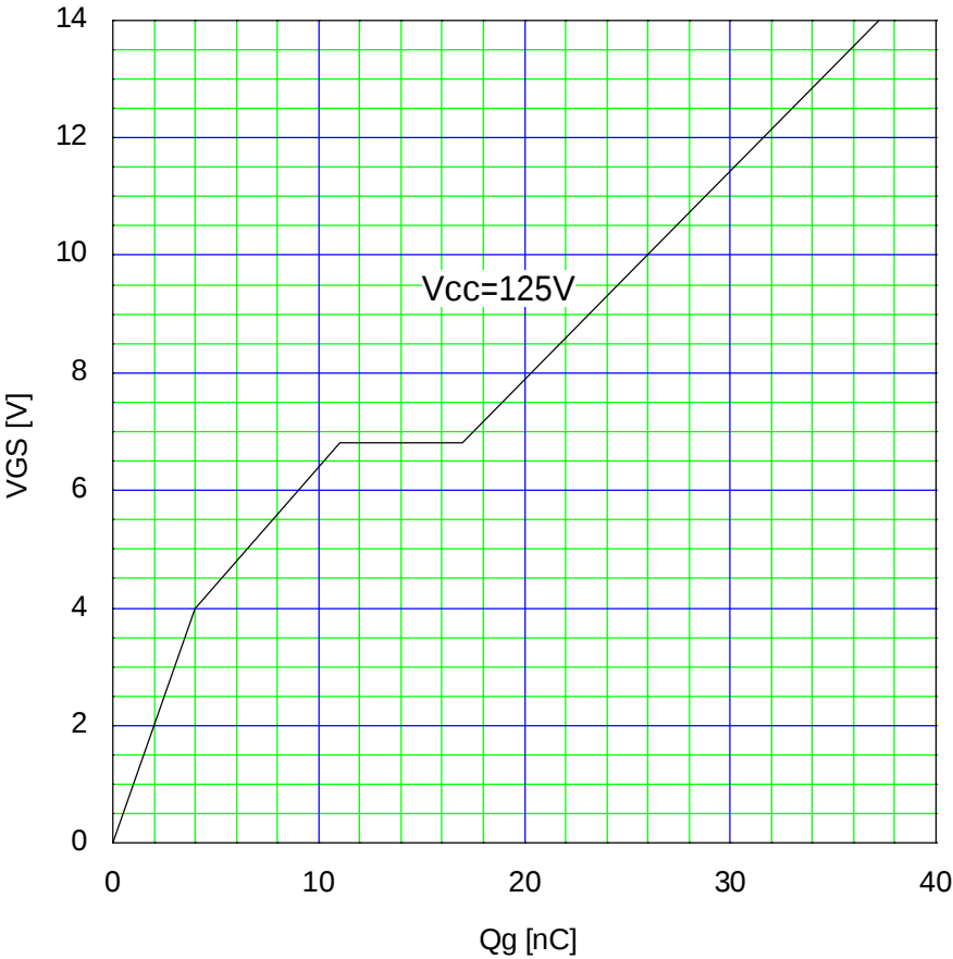
Typical Gate Charge Characteristics V_{GS}=f(Q_g):I_D=18.0A,T_{ch}=25^{\circ}C
