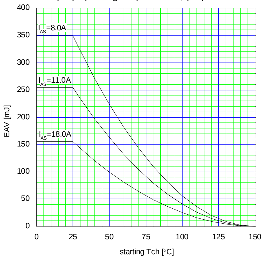
Maximum Avalanche Energy vs. starting Tch E(AV)=f(\text{starting Tch}): V_{CC}=25V, I(AV) \leq 18.0A
