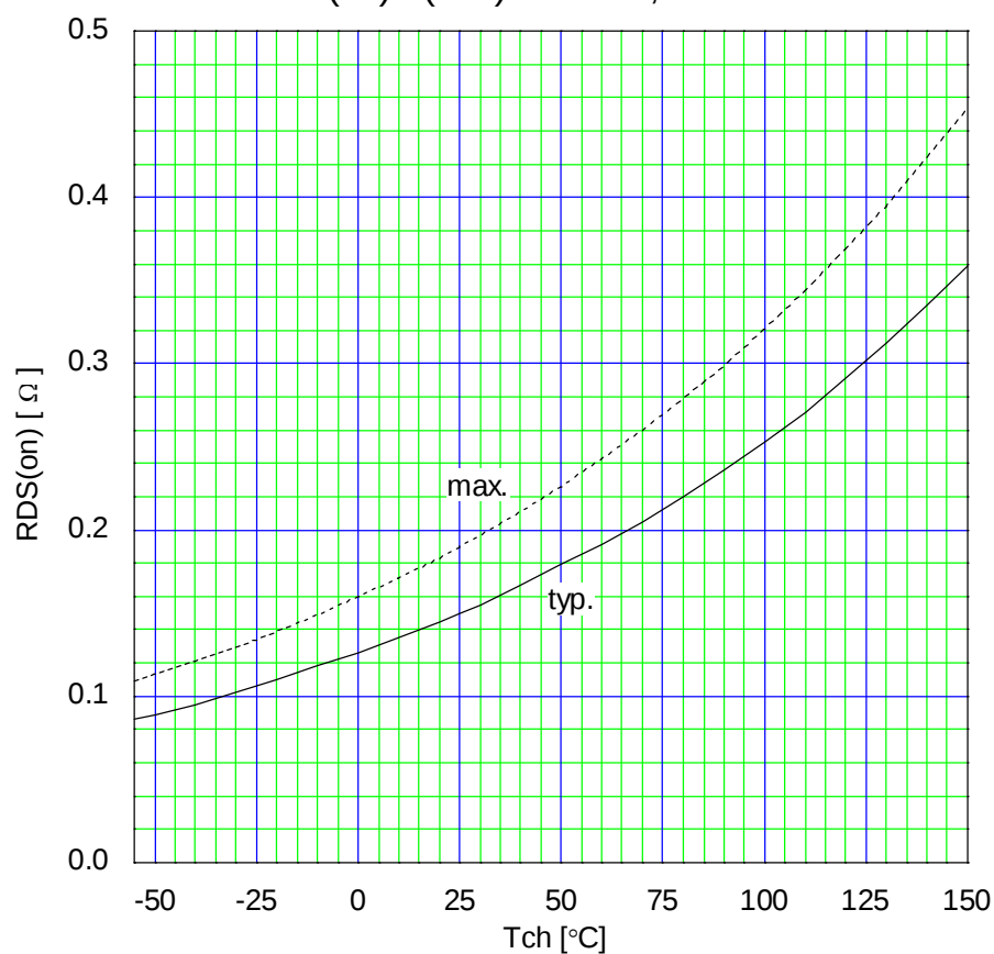
Drain-Source On-state Resistance R_{DS(on)}=f(T_{ch}):I_D=9.0A, V_{GS}=10V
