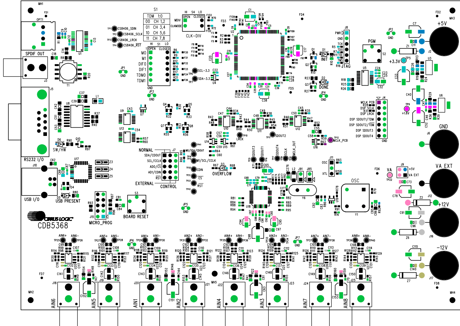
Figure 13. Top Silkscreen
