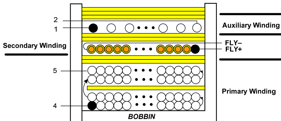
Figure 44. Transformer
