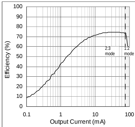
Figure 19. Efficiency vs. Output Current; V_{IN}=4.3V
