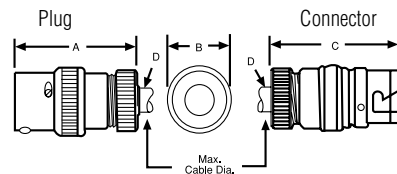
Bushing Type
