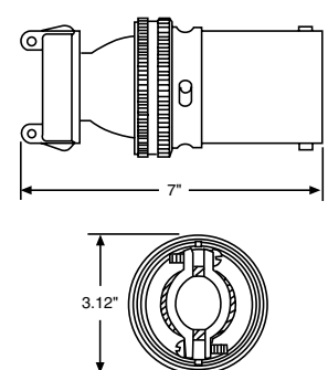
60 Amp Plug
