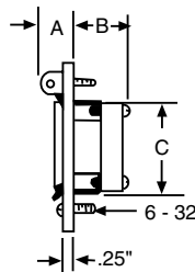
w/Box FSWS-62
