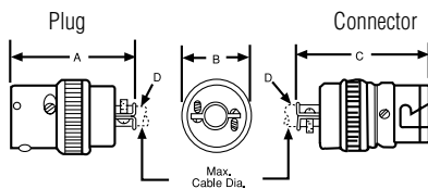
Clamp Type
