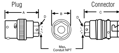
Hub Type
