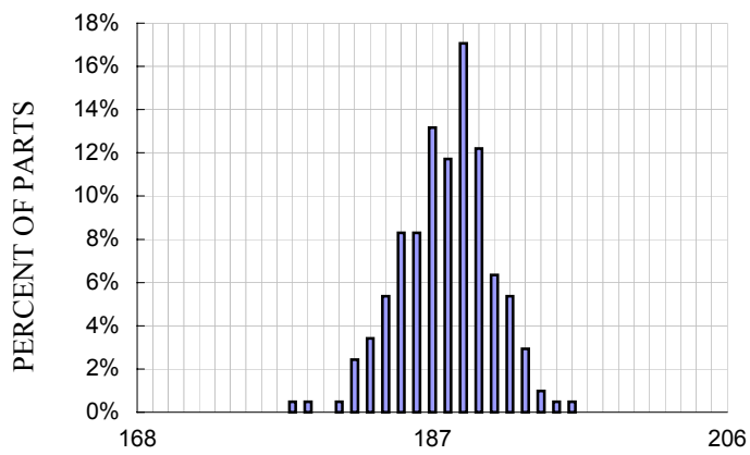
Y-axis Sensitivity Distribution at Yout, V_{DD}=3V
