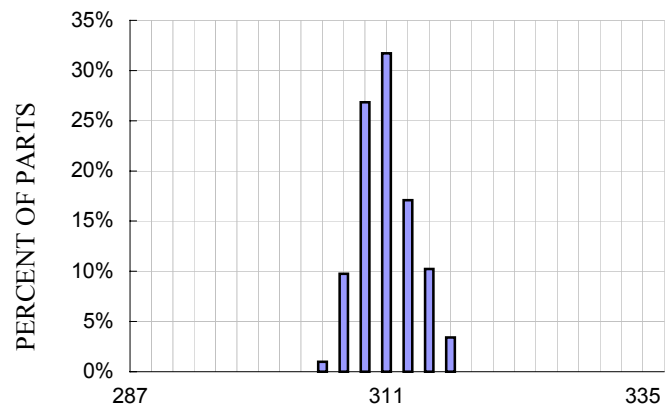
Y-axis Sensitivity Distribution at Yout, V_{DD}=5V
