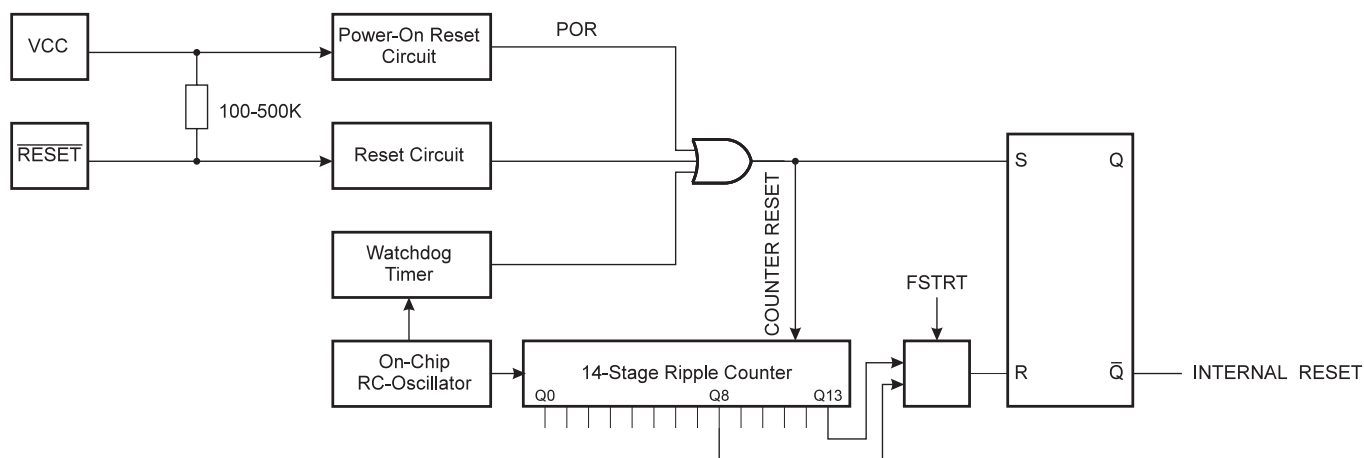
Figure 23. Reset Logic
