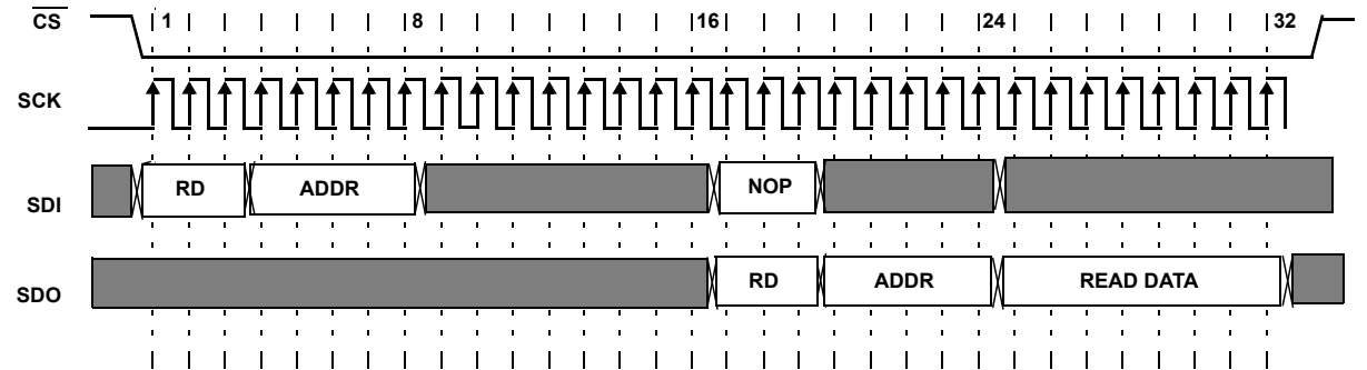
FIGURE 28. FOUR-BYTE READ SEQUENCE
