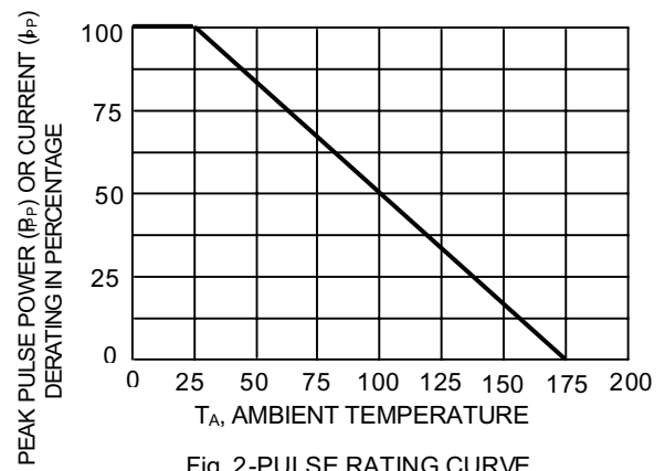
Fig. 2-PULSE RATING CURVE
