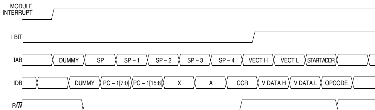
Figure 14-7. Interrupt Entry
