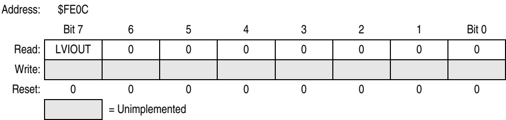
Figure 11-2. LVI Status Register (LVISR)
