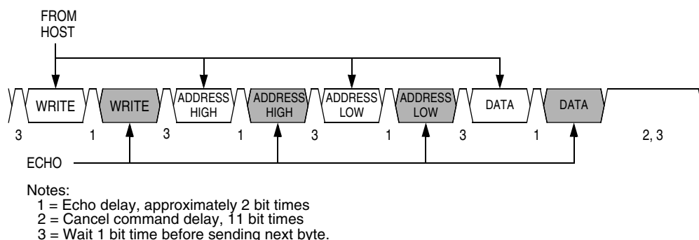
Figure 19-15. Write Transaction
