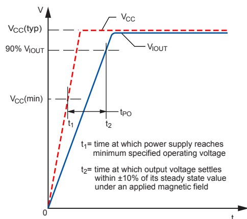
Figure 3: Power-On Time
