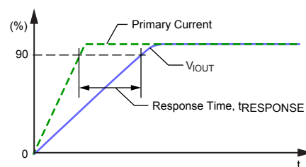
Figure 5: Response Time
