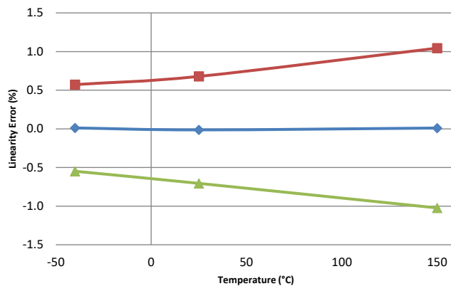
Linearity Error vs. Temperature
