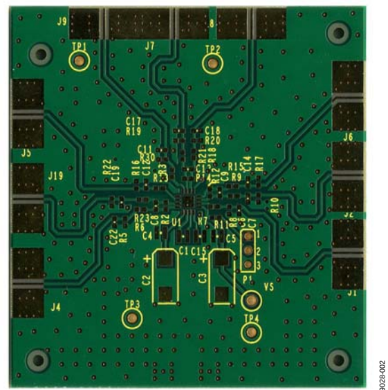
Figure 2. EB-O16CP44CP-3Z Evaluation Board, Circuit Side
