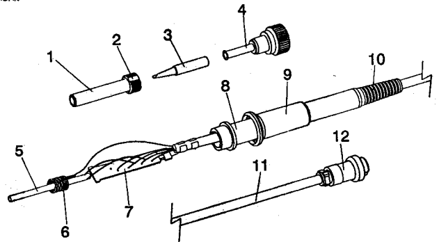
107ESD EXPLODED DRAWING
