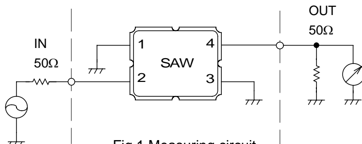
Fig.1 Measuring circuit
