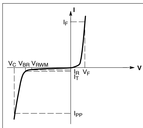
Uni-Directional TVS
